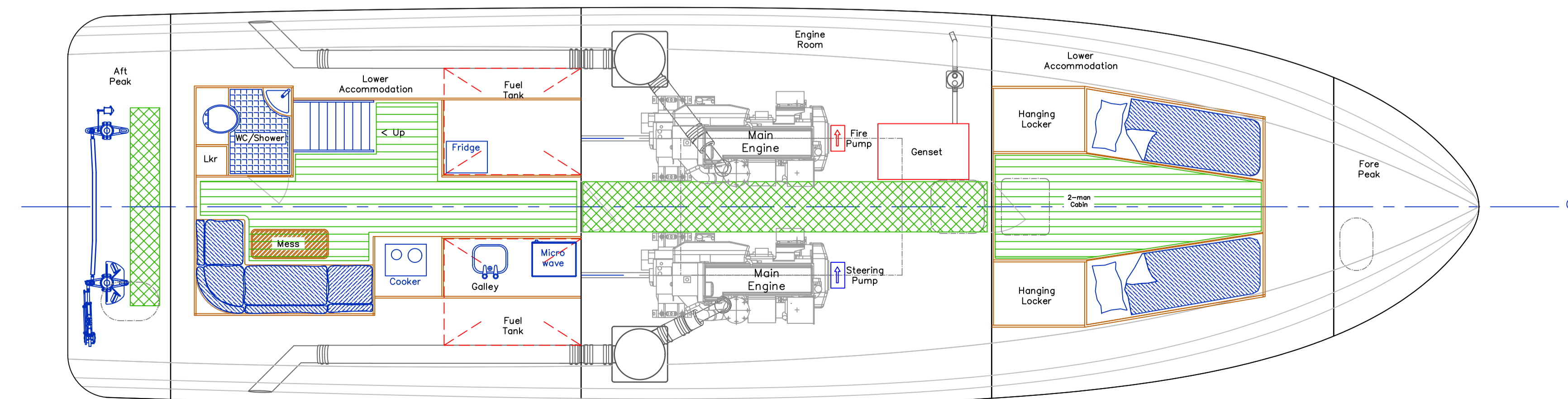
LOWER DECK PLAN
