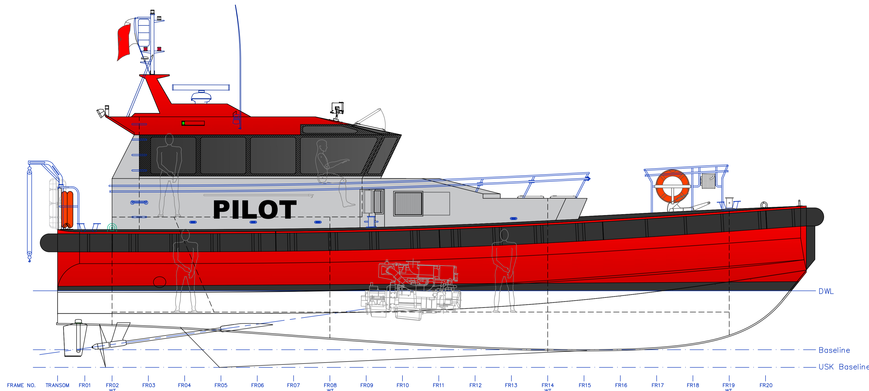
PROFILE
