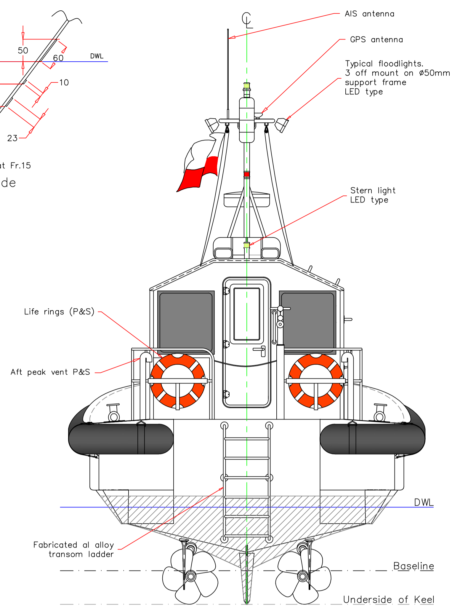
STERN VIEW
