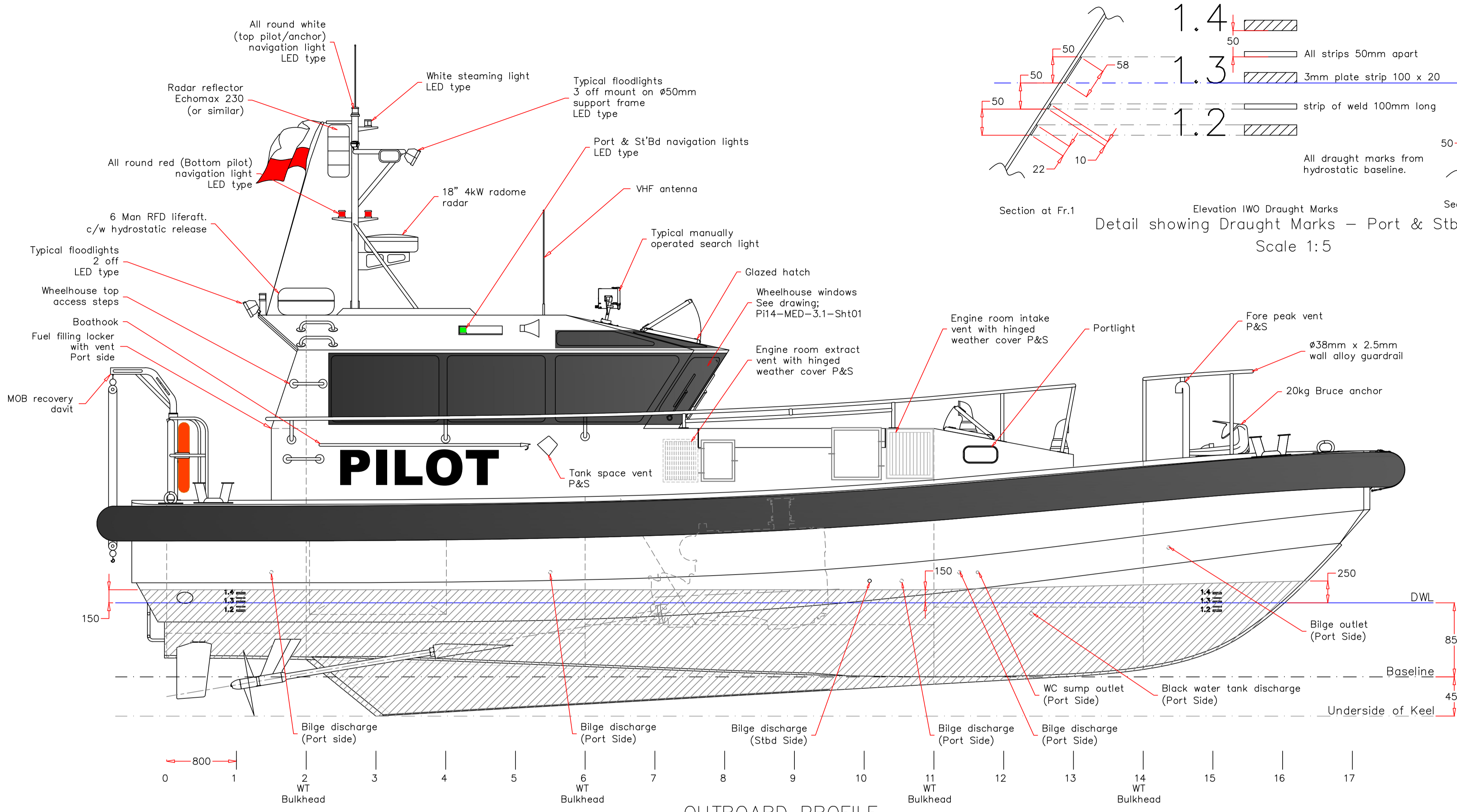
OUTBOARD PROFILE
