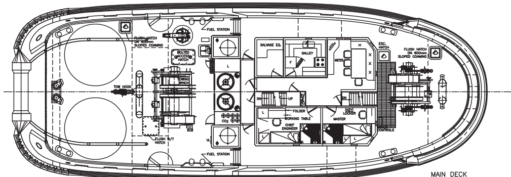
MAIN DECK
