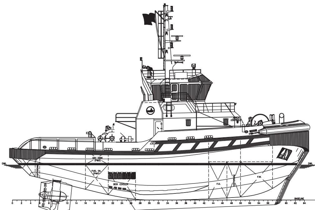
PROFILE
