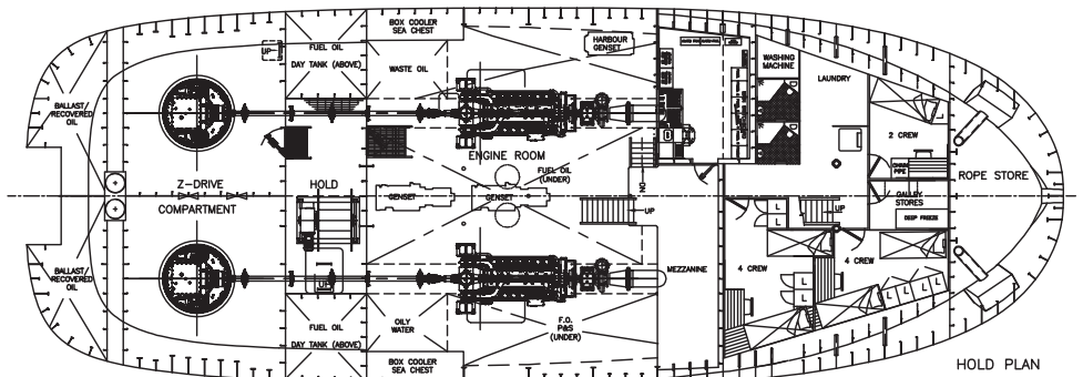
HOLD PLAN
